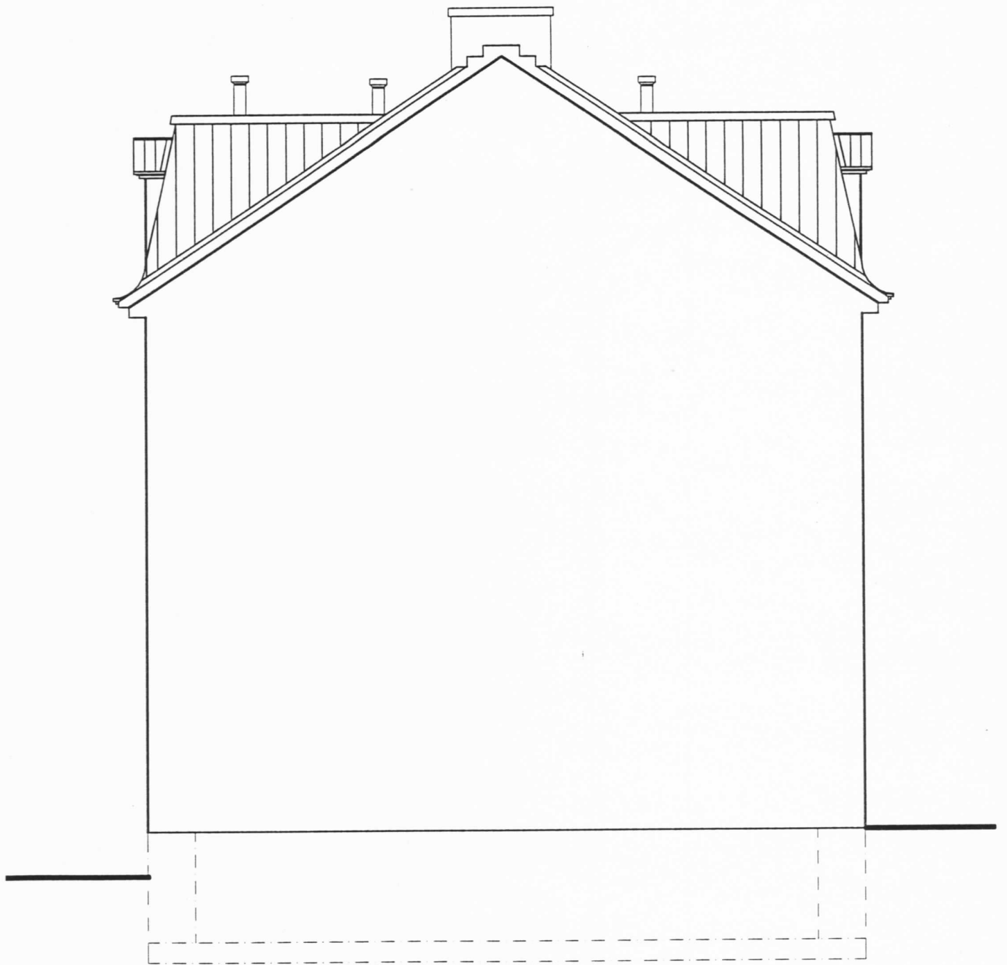
ÉLÉVATION NORD / NORTH ELEVATION
